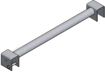
Transom Yatay-Yatay Transom Tubular Ledger & Transom Tubular Ledger
